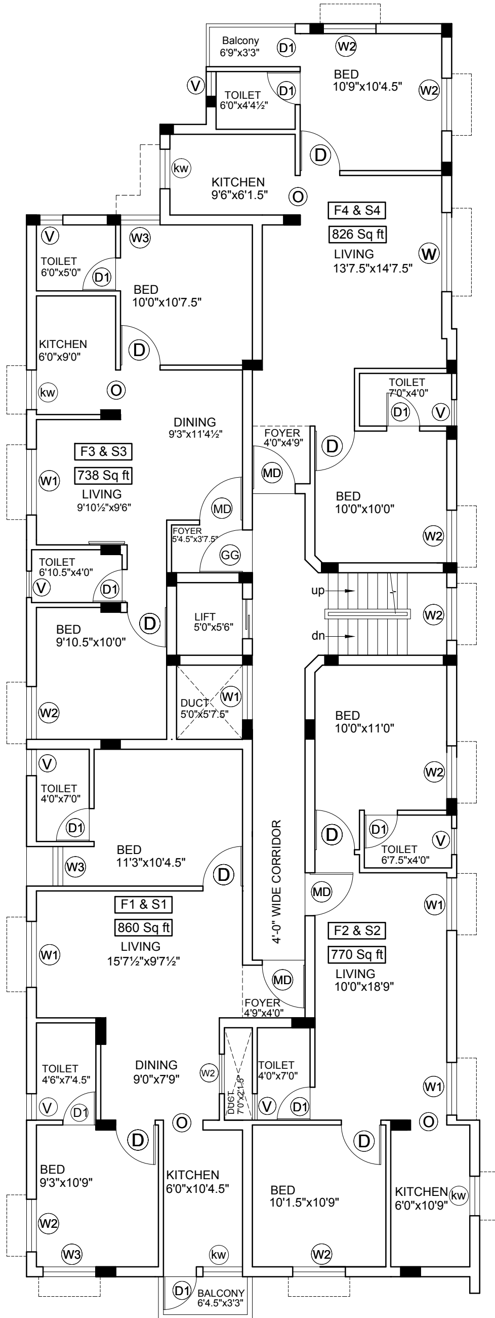
TYPICAL FLOOR PLAN (FIRST & SECOND FLOOR PLAN)
